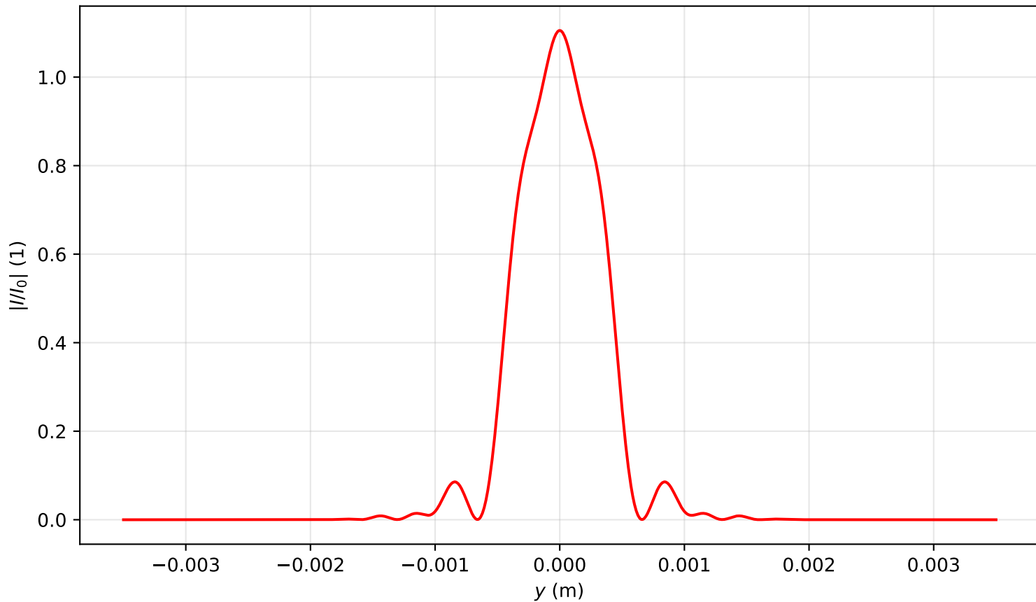
Intensity profile I(x=0, y, z=1.433)/I_0 , P_{in}=2.5P_{cr} , artificial time
